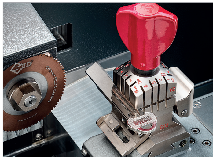
Four-sided V2 clamp (F600-F400)
