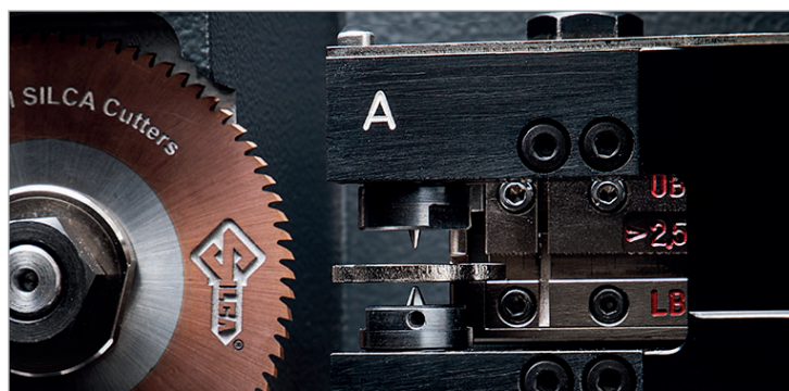
Engraving on both key sides (F900-F800-F600)
